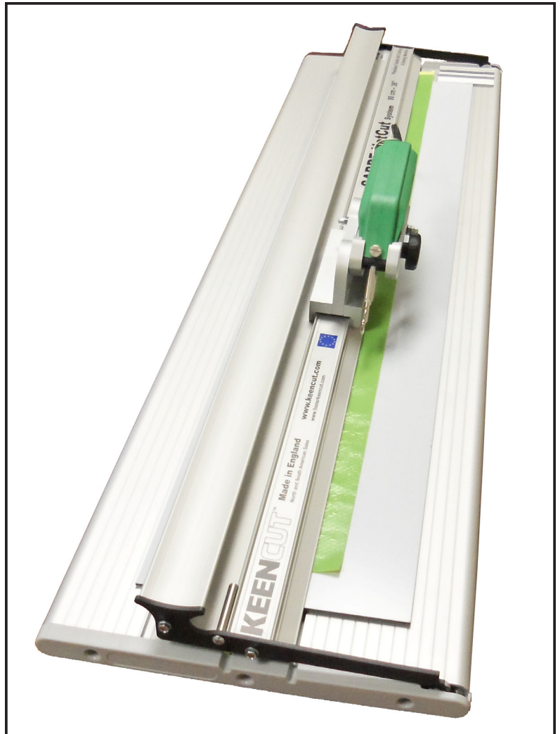
HSGM Hot Cut System. *Glass not included. 1/4" tempered glass recommended.
